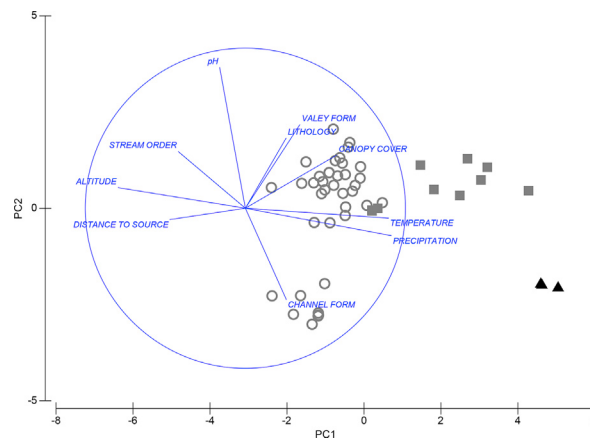
Fig. 2. Principal Components Analysis (data transformed by log x+1 and normalized) based on abiotic characteristics of Cerrado (grey open circles), Atlantic Forest (grey squares) and Amazonia (black triangles) biome sites.
