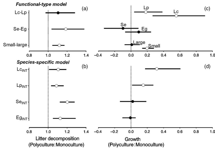
FIGURE 3 Ratio of decomposition rates between polycultures and monocultures (a, b) and difference in detritivore growth between polycultures and monocultures (c, d) for the interaction of species of similar (Lc-Lp, Se-Eg) or different body size (small-large) or for the average interaction of each species (see Figure 2 legend). The dashed line denotes the value of 1 (for decomposition) or 0 (for growth), that is, the null expectation that the polyculture value is not different from the mean value of constituent monocultures. Circles are means, and horizontal lines denote upper and lower limits of 95% nonparametric bootstrapped confidence intervals; closed circles represent intervals that do not reject the null hypothesis (i.e. do not contain the value of one or zero), and open circles represent intervals that do reject the null hypothesis
